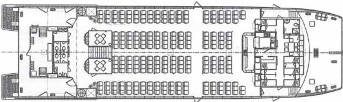
MEZZANINE DECK
