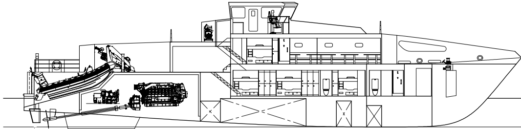
PROFILE @ CENTRELINE
